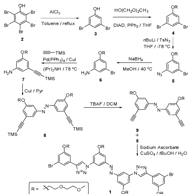
Scheme 2. Synthesis of Photoswitch 1
