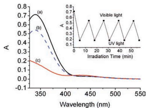
Figure 4. UV–vis spectra of (a) \mathbf{1}_{trans} ( 30 \mu\text{M} , acetone) in the presence of 4 equiv of chloride ions. (b) Irradiation with 365 nm light for 5 min, then (c) irradiation with visible light for 8 min. The insert figure reflects the changes of the absorbance at 339 nm upon alternate irradiation with UV and visible light.
