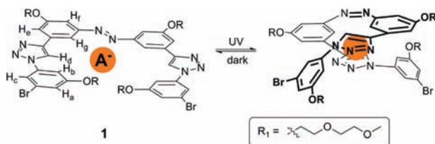
Scheme 1. Photoswitch 1 Studied Herein and Proposed Different Binding Model for Its Two Photoisomers to Anions
